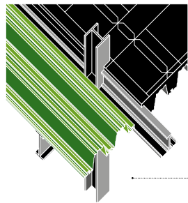
Chiodo sparato o vite autofilettante o vite automaschiante Shot nail or self-threading screw or self-tapping screw
