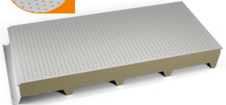
Foratura R4T6 • Rapporto vuoto/pieno 37% R4T6 Drilling • Solid/void ratio 37%
